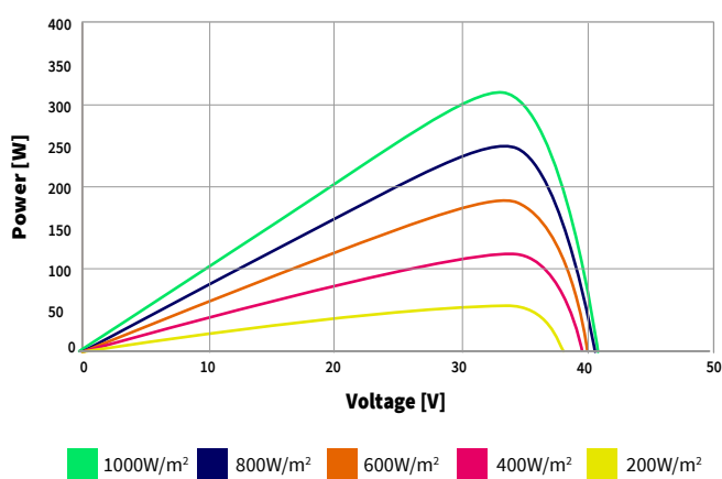
Power-Voltage Curve (375 W)
